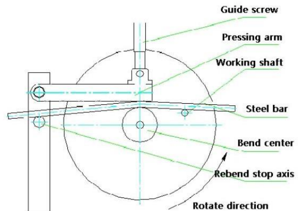
Motorized reverse bending test
